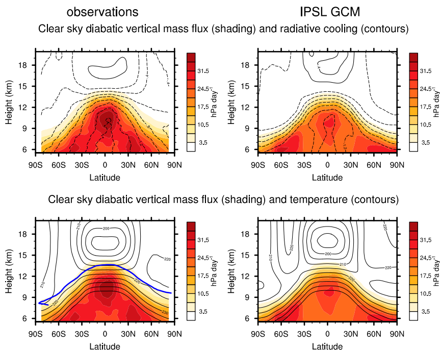
Fig. 1. (Top) Clear-sky radiative cooling (contours) overlaid with the diabatic vertical mass flux calculated as -Q_r/S (shading). (Bottom) Clear-sky diabatic vertical mass flux (shading) superposed on temperature (contours). The thick blue line in Bottom Left indicates the 20 ppmv isopleth based on the MLS water vapor data. Results in the Left are derived from observations. Results in the Right are derived from the IPSL general circulation model (GCM). Observations are based on CloudSat clear-sky cooling rates and the CloudSat ECMWF-AUX product.
