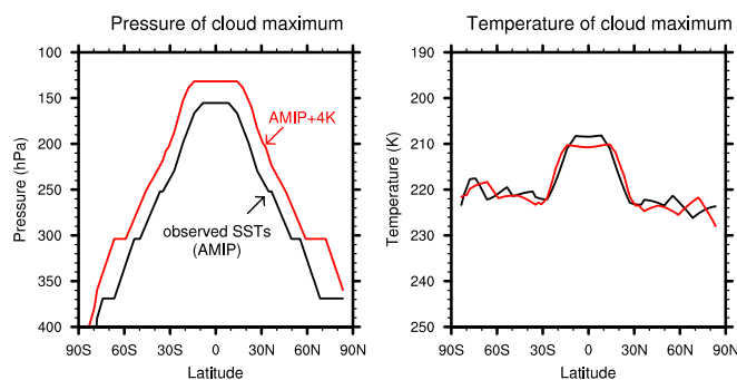
Fig. 5. The pressure ( Left ) and temperature ( Right ) of the maximum in cloud fraction as a function of latitude for climate model output from the IPSL general circulation model (GCM). The black lines indicate results from a simulation forced with time-varying sea surface temperatures (SST) from 1979 to 2008 (observed SSTs; AMIP). The red lines indicate results from a simulation where sea surface temperatures are increased everywhere by 4 K relative to their 1979–2008 values (AMIP+4K). Results are smoothed with a latitudinal running mean filter for display purposes only.
