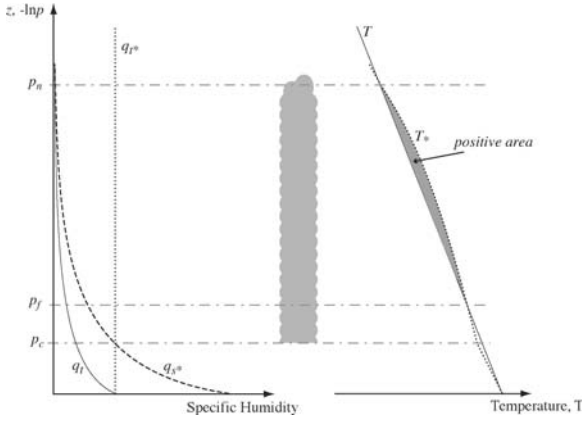
Figure 3 State diagram for an atmosphere stable to infinitesimal, but unstable to finite amplitude, displacements of near surface air.
