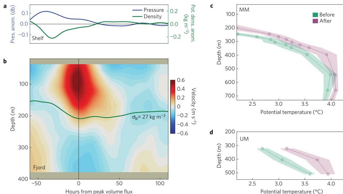
Figure 2 | Structure and impact of velocity pulses. a , Composites of potential density anomaly and bottom pressure anomaly (both 26-h low-pass filtered, with 30-day low-pass signal removed) from shelf mooring. b , Composite of velocity at mid-fjord with contour of \sigma_{\theta} = 27.0 \text{ kg m}^{-3} from composite of mid-fjord potential density (30-day low-pass signal removed and mean added back). Positive velocities indicate flow up-fjord, towards the glacier. The composites in a , b are of various records over the 16 strongest velocity pulses (defined by an up-fjord volume flux in the upper layer exceeding 3.7 \times 10^5 \text{ m}^3 \text{ s}^{-1} ; Methods and Fig. 3a). c , d , Potential temperature profiles during four-day periods preceding and following a strong up-fjord flow (indicated with grey vertical lines in Fig. 1c, d) in the AW layer at mid-fjord mooring (MM; c ) and upper-fjord mooring (UM; d ). Circles show average temperature at the instrument during each period; shading indicates the 95% range of all measurements over this period.
