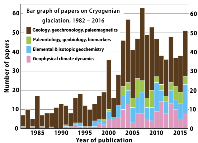
Fig. 28. Bar graph of peer-reviewed papers on Cryogenian glaciation by discipline and year, 1982 to 2016. Papers are assigned to one of four disciplinary categories. Note the relative growth of geophysical and geochemical papers after 1996 and geobiological papers after 2002. From the 1870s through the 1980s, research on “eo-Cambrian” glaciation was almost exclusively geological (55). The 70 chapters by various authors in the work of Amdur et al. (175) are not tallied here. Forward modeling papers (in all categories) account for only ~25% of the current total.
