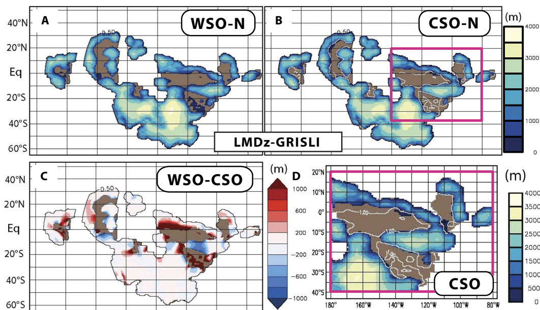
Fig. 11. Sensitivity of ice sheets on Snowball Earth to precession-like forcing (100). Same coupled atmosphere–ice-sheet model as in Fig. 10, with CO 2 = 20 mbar. Model equilibrated to northern-hemisphere (A) warm (WSO-N) and (B) cold (CSO-N) summer orbits. Orbits were switched every 10 ky. Scale bars are ice thickness (in meters), and brown areas are ice-free. (C) Difference in local ice-sheet mass balance, with red and blue indicating positive and negative mass balance, respectively, in the WSO-N relative to CSO-N. Note the hemispheric asymmetry as expected for precession, but areas of positive and negative mass balance coexist in both hemispheres at low latitudes, expressing the sensitive response of the hydrologic cycle. Positive mass balance in the war-summer hemisphere is related to prescribed change in eccentricity. (D) Expanded sector (magenta box) under CSO-N with white lines indicating ice margins under WSO-N for comparison. Ice margins migrate <math><5^\circ</math> (550 km) on the precessional time scale.
