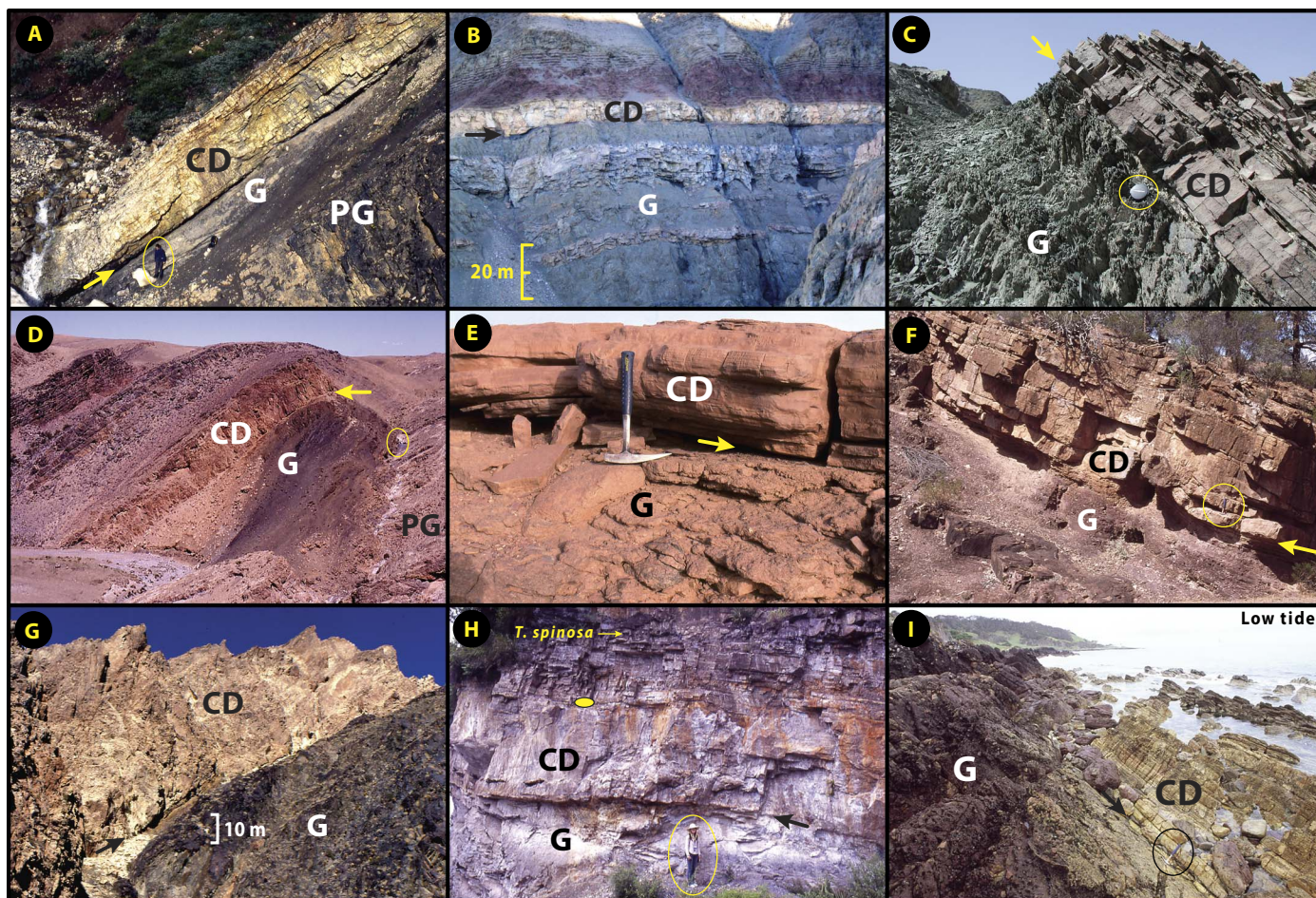
Fig. 23. Global distribution of sharp-based Marinoan postglacial cap dolostones. Distribution of Marinoan cap dolostones over 110^\circ paleolatitude, from South China at 45^\circ\text{N} (H) to West Africa at 65^\circ\text{S} (E) (Fig. 5A), records an anomalous state of carbonate oversaturation in the surface ocean despite extreme \text{CO}_2 acidification in the Snowball aftermath (73, 74, 84–91). Other Marinoan cap dolostones are imaged in Figs. 7C and 25B. PG, preglacial carbonate strata; G, glacial-periglacial deposits; CD, cap dolostone. Arrows mark sharp basal contacts. (A) Ravenstroat Formation (CD) on Stelfox Member, Ice Brook Formation (G), and Keele Formation (PG), Arctic Red River, Mackenzie Mountains, Northwest Territories, Canada (409, 416, 499). (B) Basal Canyon Formation (CD) on Storeelv Formation (G), Tillitekløft, Kap Weber, Kejser Franz Joseph Fjord, East Greenland (139, 334). Resistant layers of quartz sandstone within glacial diamictite were eroded from un lithified preglacial marine sandstones. Photo courtesy of E. W. Domack. (C) Basal Zhamoketi Formation (CD) on Tereeken Formation (G), Yukkengol, Quruqtagh, Xinjiang, China (500). A lens cap is used for scale. Photo courtesy of S.-H. Xiao. (D) Basal Ol Formation (CD) on Khongor Formation (G) and Taishir Formation (PG), Khongoryn, Zavkhan, western Mongolia (143, 501). (E) Amogjar unit (CD) on Jbeliat Group (G), Atar, Adrar, Taoudeni Basin, Mauritania (161). (F) Nuccaleena Formation (CD) on Elatina Formation (G), Elatina Creek, Central Flinders Ranges, South Australia (427). (G) Sentinel Peak Member (CD) of the Noonday Dolomite on Wildrose Member (G) of the Kingston Peak Formation, Goller Wash, Panamint Range, Death Valley area, eastern California, USA (469, 470). (H) Basal Doushantuo Formation (CD) on Nantuo Formation (G), Huajipo section, Yangtze Gorges, northern Hunan, South China (417). Tianzhushania spinosa arrow indicates the first appearance of chert nodules preserving diapause cysts containing eggs and embryos of stem-group metazoans (502, 503). The yellow oval marks a volcanic ash layer yielding zircons dated at 635.2 \pm 0.5 Ma (57). (I) Cumberland Creek Dolostone (CD) on Cottons Breccia (G), Grimes Creek, King Island, Tasmania (504). Igneous zircons from the topmost meter of the Cottons Breccia are dated at 636.41 \pm 0.45 Ma (59).
