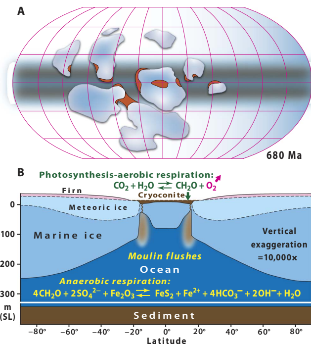
Fig. 18. Cryoconite ponds and cryoconite meltwater flushing on Snowball Earth (297). (A) Global paleogeography during the Sturtian cryochron at 680 Ma (34). Brown continental areas schematically indicate dry-valley dust sources (100). Gray areas in the low-latitude sublimation zone of the sea glacier are schematic cryoconite ponds. (B) Snapshot of a 2D ice-flow model of a Snowball Earth with a global dust accumulation rate of 10 \text{ m My}^{-1} (168). Dark cryoconite and exposed marine ice make sublimative ice warm and thin. Hemispheric asymmetry at low latitude reflects unsteady, quasi-periodic, reciprocal ice surges from the respective subtropics in the model. Flushing of meltwater and cryoconite through moulin is shown schematically. The apparent ice walls at 18^\circ latitude have actual slopes of 1 \text{ m km}^{-1} . Organic production is nearly balanced by aerobic respiration within cryoconite holes and ponds. Flushed cryoconite organic matter is subject to anaerobic respiration in the water and sediment columns. Fe(III) and sulfate are sourced from the flushed cryoconite and sub-ice-sheet weathering. If anaerobic respiration is incomplete, organic matter is buried and O_2 is added to the atmosphere. SL, sea level.
