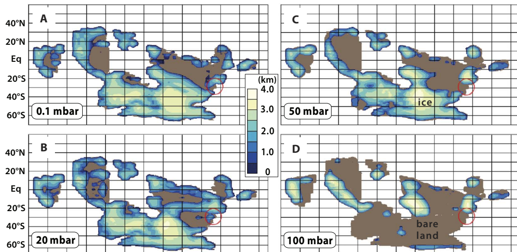
Fig. 10. Ice-sheet recession on Snowball Earth with rising CO 2 (100). Results from experiments with the atmospheric component of GCM LMDz, coupled to ice-sheet model GRISLI, in Cryogenian paleogeography with prescribed orography under Snowball conditions with present-day orbit and CO 2 = 0.1 mbar (A), 20 mbar (B), 50 mbar (C), and 100 mbar (D). Scale bar is ice-sheet thickness (in kilometers), and brown areas are ice-free. Red circles indicate the study location in Svalbard. Large base-level rise associated with Marinoan deglaciation may imply that more ice was available for melting than in (D), consistent with terminal deglaciation at less than 100 mbar of CO 2 .
