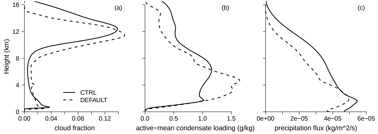
Figure 2. (a) Cloud fraction, (b) updraft-mean non-precipitating cloud condensate q_c , and (c) precipitation flux in the CTRL and DEFAULT simulations. For DEFAULT, q_c includes non-precipitating cloud liquid and cloud ice and the precipitation flux includes rain, snow, and graupel. For CTRL, neither q_c nor the precipitation flux are differentiated into liquid and ice subspecies because of the simple microphysics scheme used in that simulation.
