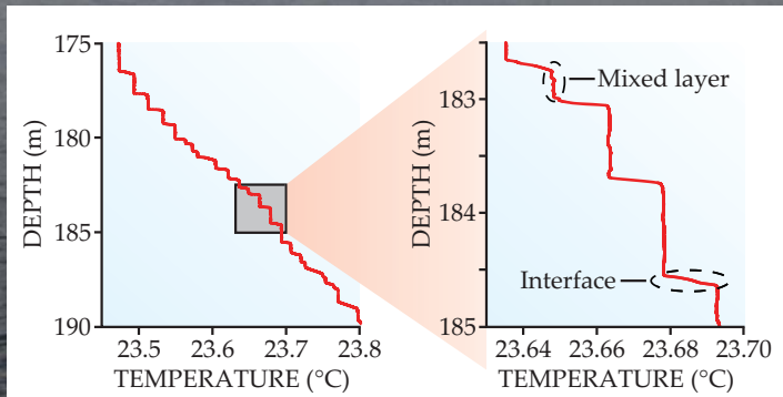
An aquatic staircase in the tropics. The background image shows Lake Kivu and the smoking Nyiragongo volcano, located in tropical Africa. Deep springs inject warm, salty water below the lake surface and create the conditions needed for one of the double diffusion processes described in the text. As a result of that double diffusion, the temperature–depth profiles shown in the graphs exhibit a staircase structure. (Photograph by Jeff Carpenter; data courtesy of Tobias Sommer and Alfred Wüest.)
