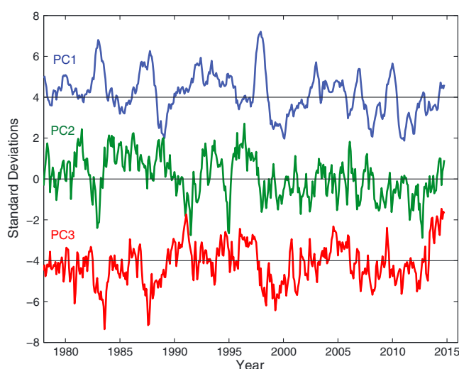
Figure 2. Time series of the principal components of the first three EOFs of monthly mean Pacific SST poleward of 30°S as shown in Figure 1. Only values from January 1979 to January 2015 are shown. Units are standard deviations. Values are offset by four standard deviations for clearer viewing.
