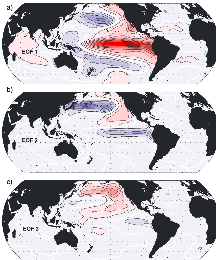
Figure 1. The regressions of monthly mean anomalies of global SST onto the first three EOFs of SST for the ocean area 30°S–65°N, 120°E–105°W and the period from January 1900 to July 2014. Contour interval is 0.1°C. Positive values are red, negative values are blue, and the zero contour is white. Robinson projection from 60°S to 60°N.
