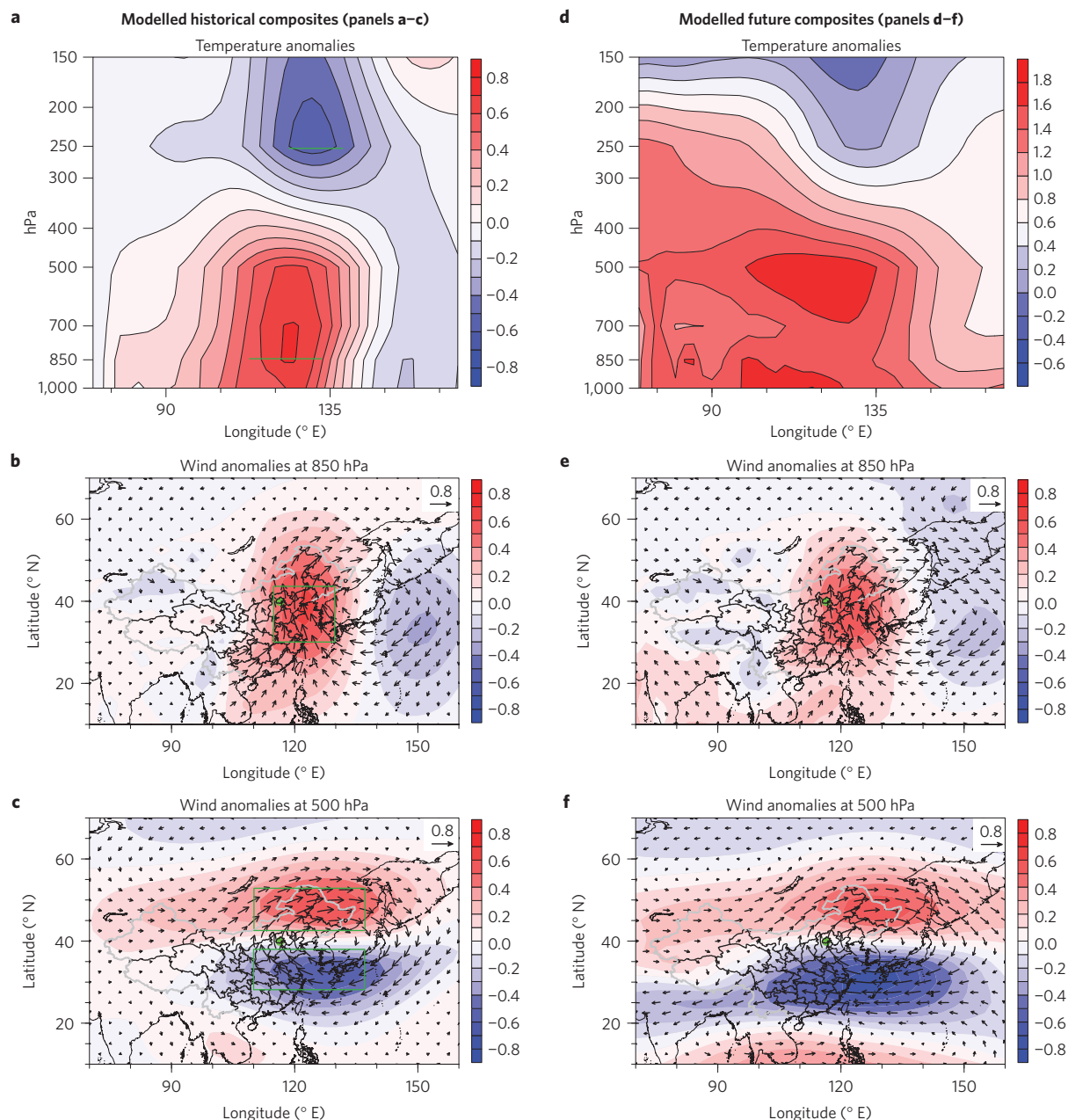
Figure 4 | Simulated winter severe haze weather conditions near Beijing (116.4° E, 39.9° N). a–c , Composites for days with HWI > 0 in terms of anomalous temperatures throughout the atmospheric column in an east–west section ( a ), anomalous flow vectors at 850 hPa for V850 (shading indicates meridional flow) ( b ), and anomalous flows at 500 hPa for U500 (shading indicates zonal flow) ( c ), for the historical climate (1950–1999). d–f , The same as a–c , respectively, but for future climate (2050–2099), aggregated over 15 models. All anomalies are referenced to the historical daily climatology and normalized by the historical standard deviation to facilitate comparison between the historical and future climate. The green dot denotes the location of Beijing. The green boxes denote regions for averages.
