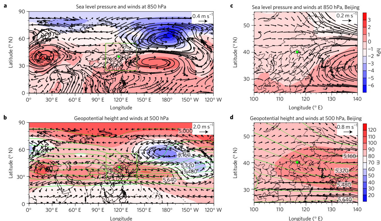
Figure 5 | Simulated multi-model ensemble mean state changes in boreal winter mean circulation. a,b, Changes in 850 hPa wind vectors ( \text{m s}^{-1} ) and sea level pressure (hPa) ( a ), and 500 hPa wind vectors ( \text{m s}^{-1} ) and 500 hPa geopotential height (m) ( b ). These changes are taken as the difference between the future and the historical climate (2050–2099 minus 1950–1999). c,d, The same as a,b , respectively, but with a focus on the Beijing area. These changes are consistent with an upward trend of the Arctic Oscillation and a weakening East Asia winter monsoon, both contributing to anomalous southerly winds near Beijing. Green contours in b and d are simulated mean 500 hPa geopotential height (m) under the historical climate (1950–1999). The green boxes denote regions for focus in c and d .
