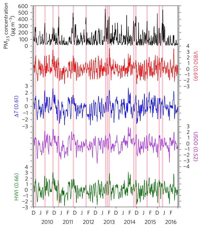
Figure 2 | Time series of 2009–2015 normalized observed boreal winter daily \text{PM}_{2.5} ( \mu\text{g m}^{-3} ) and normalized daily weather conditions near Beijing. V850 (red), \Delta T (blue) and U500 (purple) (see text for their definitions) are normalized by their respective standard deviations. Occurrences when \text{PM}_{2.5} (black) reached a high concentration are highlighted. Highlighted slots illustrate the correlations between weather time series, and with \text{PM}_{2.5} as listed in brackets near the y-axis labels. The haze weather index (HWI; green) is constructed by adding the above three weather time series, and scaling by the standard deviation of the combined time series.
