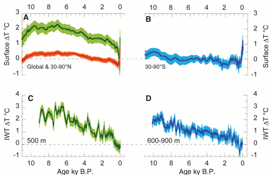
Fig. 2. Comparison between Holocene reconstructions of surface and intermediate-water temperatures. (A) Global (red) and 30^\circ\text{N} to 90^\circ\text{N} (green) surface temperature anomalies, (B) 30^\circ\text{S} to 90^\circ\text{S} surface temperature anomalies (24), (C) changes in IWT at 500 m, and (D) changes in IWT at 600 to 900 m. All anomalies are calculated relative to the temperature at 1850 to 1880 CE. Shaded bands represent \pm 1 SD. Note the different temperature scales.
