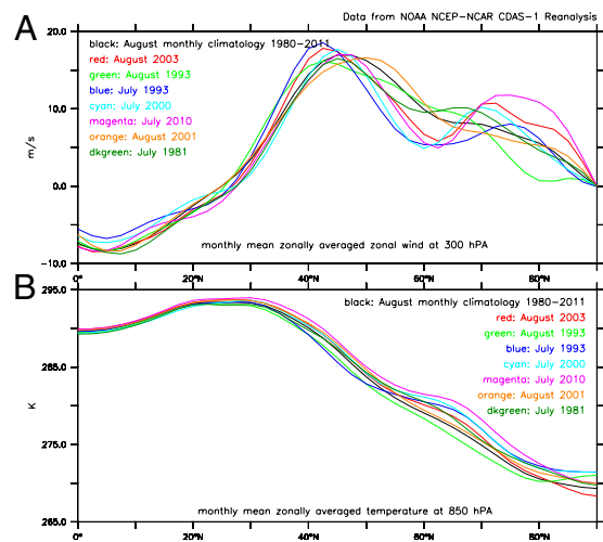
Fig. 5. Latitudinal distributions for zonally averaged monthly zonal wind (in meters per second) and temperature (in kelvins) for extreme August 2003, July 2010, July 2000, and July 1993 in comparison with nonresonance July 1981, August 1993, August 2001, and the 1980–2011 climatology. (A) Zonally averaged zonal wind at 300 hPa for August 2003 (red), July 2010 (magenta), July 2000 (cyan), July 1993 (blue), July 1981 (dark green), August 1993 (green), August 2001 (orange), and the 1980–2011 climatology (black). (B) Same as A but for zonally averaged temperature at 850 hPa.
