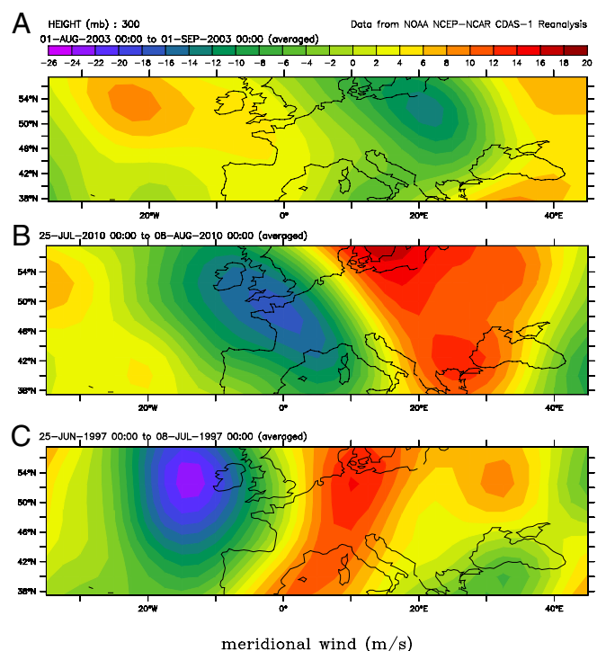
Fig. 1. Maps of the meridional winds (in meters per second) at 300 hPa over the North Atlantic–European sector during the three recent summer extremes in Europe. Shown are maps for (A) the record European summer heat wave in August 2003; (B) the most devastating phase of the Russian heat wave, July 25 to August 7, 2010; and (C) the most destructive episode of the Great European Flood, June 25 to July 7, 1997.
