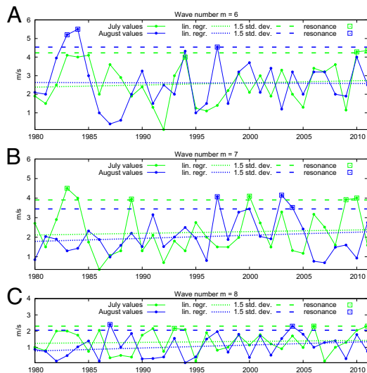
Fig. 3. The 1980–2011 time series for the amplitudes (in meters per second) of monthly Fourier components of meridional wind at 300 hPa averaged over the (37.5–57.5)°N latitudinal belt. The respective amplitudes are shown for the wave components with zonal wave numbers m = 6 (A), m = 7 (B), and m = 8 (C) for July (green) and August (blue). The squares in each plot mark the amplitudes for those months with the quasisresonance conditions for the above wave components. In each plot, the inclined dotted straight lines display the linear regressions for the appropriate monthly time series, whereas the horizontal dashed lines depict 1.5 SD from the respective 1980–2011 monthly climatology.
