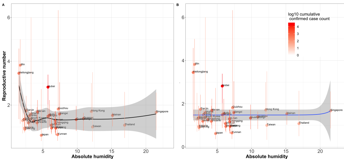
Figure 1: Estimated reproductive numbers R_{proxy} for COVID-19 plotted as a function of absolute humidity by province. 87% confidence intervals are displayed as vertical lines and were obtained from the collection of R_{proxy} calculated in subsequent time windows of length d for each location. Given the short time length of the current epidemic outbreak, an average of only 15 R_{proxy} values were calculated per location. Loess regression is shown to the left and exponential fit is shown to the right.
